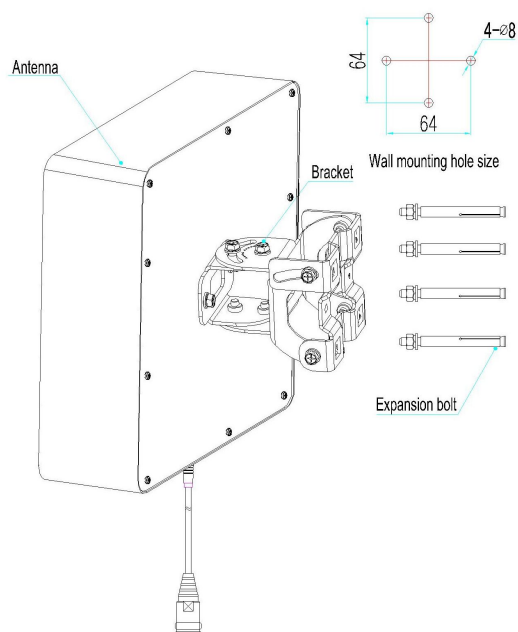
Wall Installation
